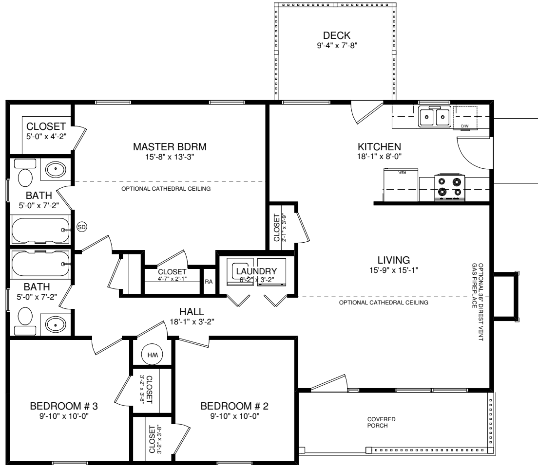
OPTIONAL FULL PORCH PLAN
