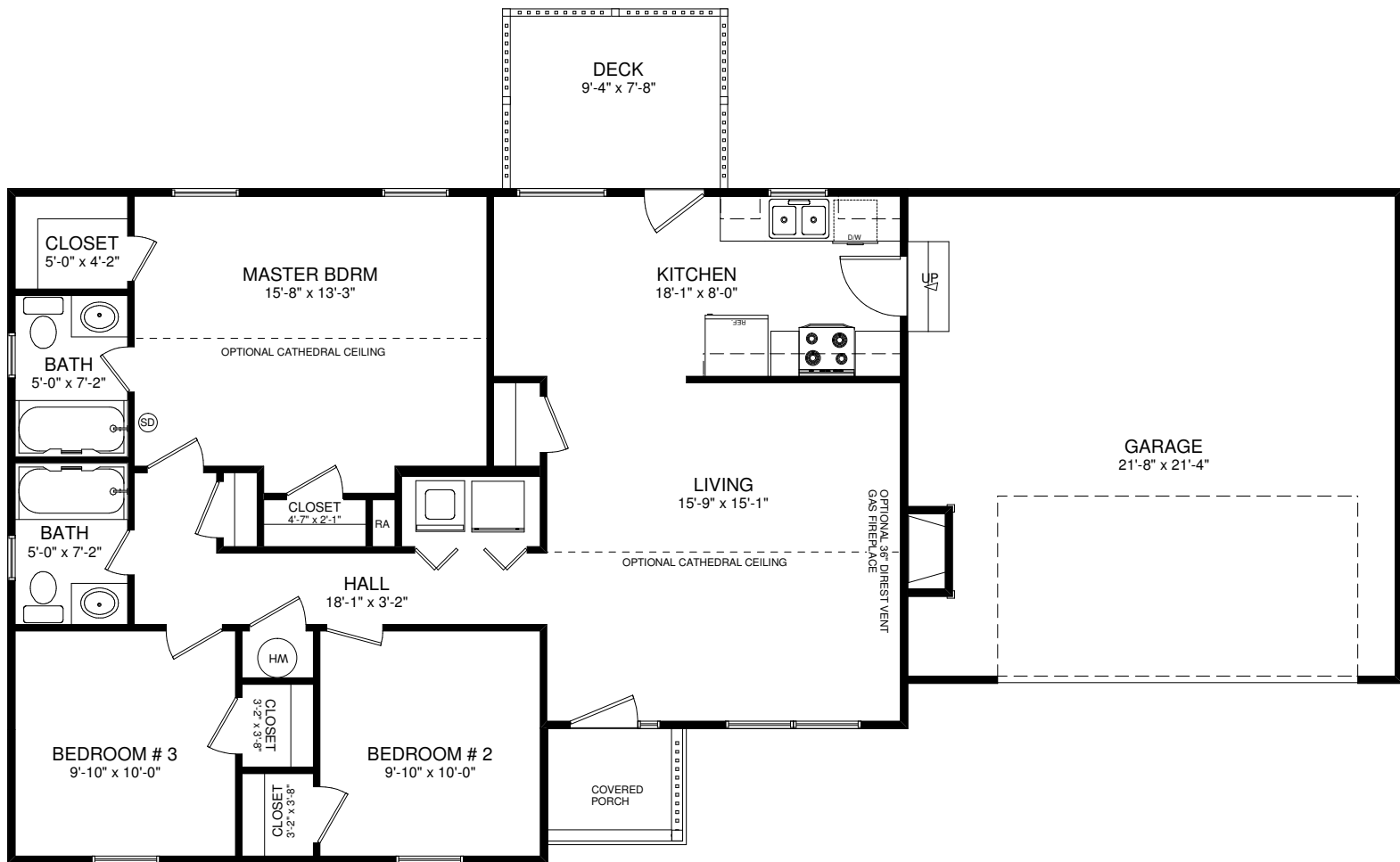
OPTIONAL FRONT LOAD GARAGE PLAN
