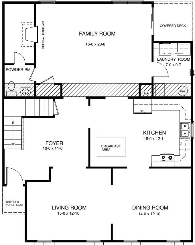
1ST FLOOR
