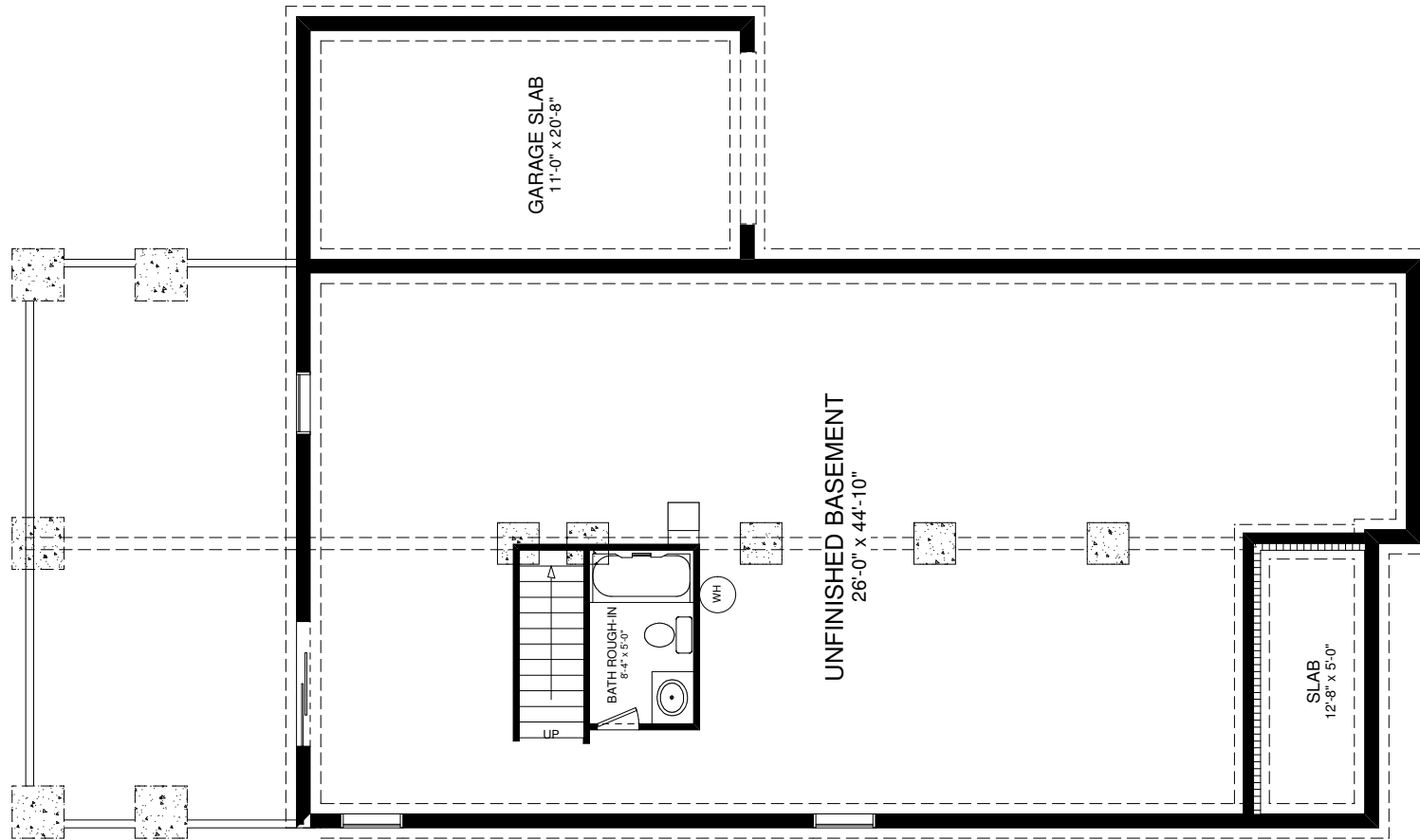
FOUNDATION PLAN
