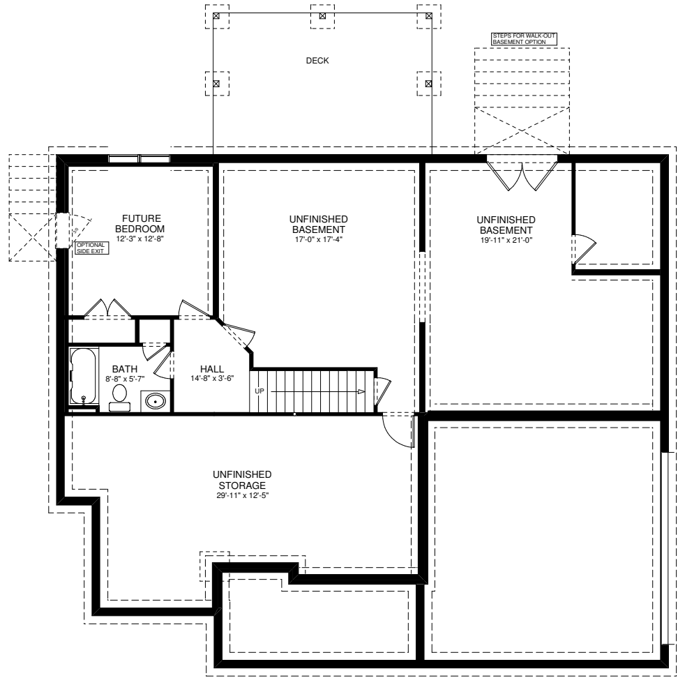
FOUNDATION PLAN
