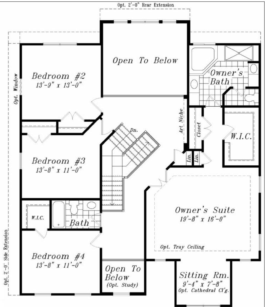
Second Floor Brochure Plan
